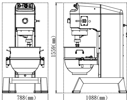
(SP-A80H/SP-B80H) DIMENSION
